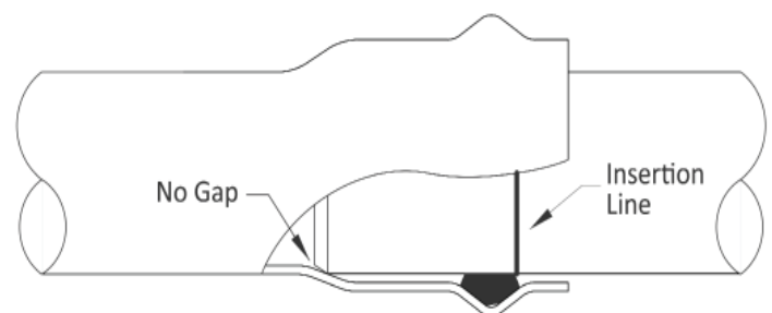
Figure 2: Over-Inserted Spigot
